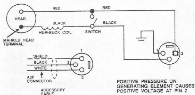
FIGURE 2 — Wiring Diagram
