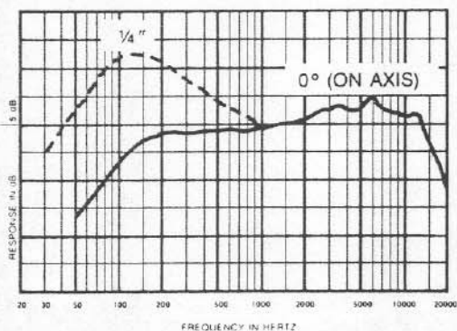
FIGURE 3 — Frequency Response
