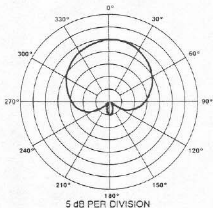
FIGURE 4 — Polar Response at 1,000 Hz
